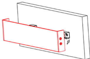
5. Install the profile with the clips
