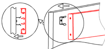
5. Mounting the fixture to the clip
