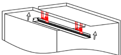
B5. Mounting the fixture with spring clips
